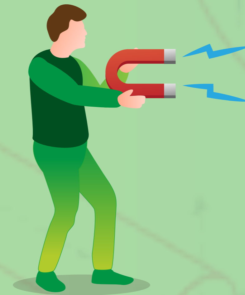
Magnetism
